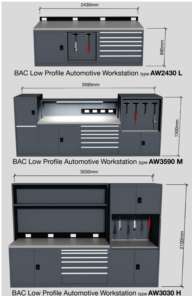
BAC Low Profile Automotive Workstation with stainless steel benchtop
